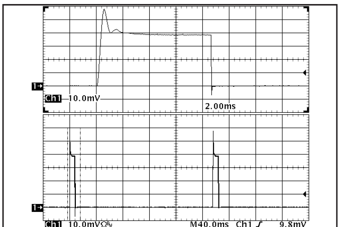
Figure 18: Load current ( 5\ \text{A}/\text{div} ) as a function of time when the converter attempts to turn on into a 1\ \text{m}\Omega short circuit. Top trace ( 2\text{ms}/\text{div} ) is an expansion of the on-time portion of the bottom trace.
